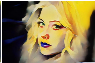
(f) AesUST
