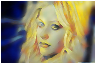
(c) AesPA-Net
