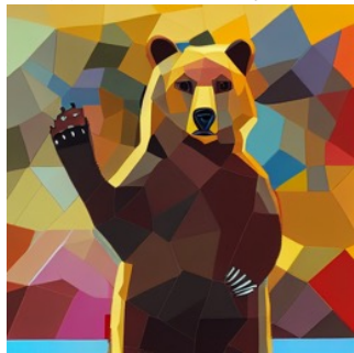
(a) DreamStyler
