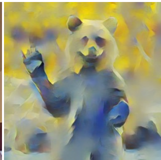
(c) AesPA-Net
