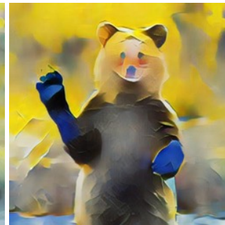
(f) AesUST
